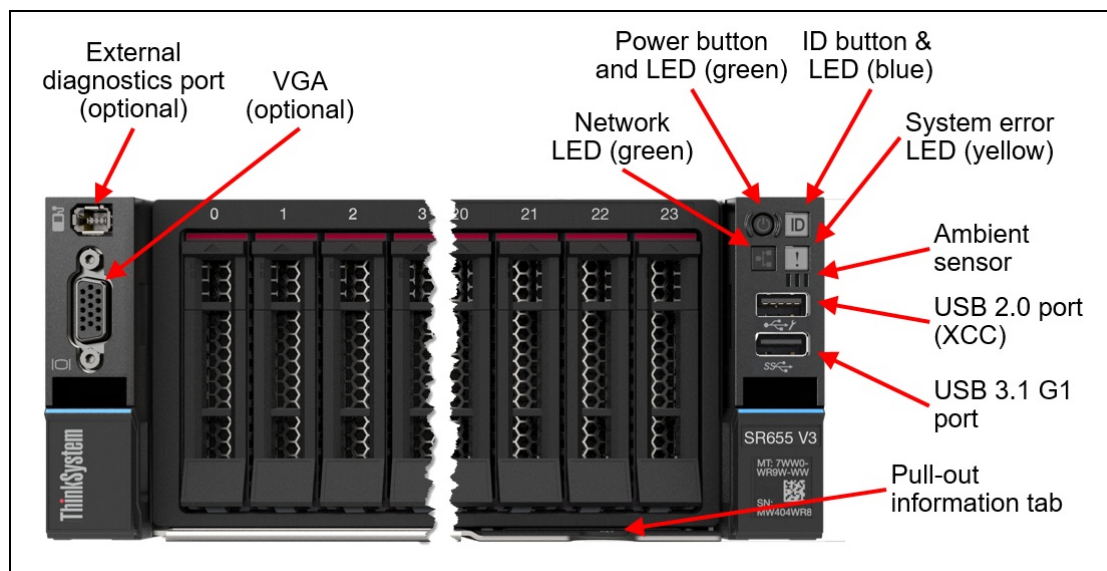
Figure 21. Front operator controls are on the left and right side of the server
