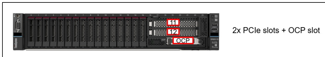
Figure 16. SR655 V3 front slots
