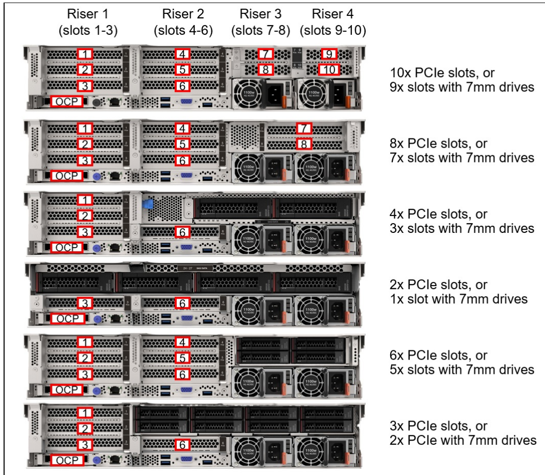
Figure 15. SR655 V3 rear slot configurations
