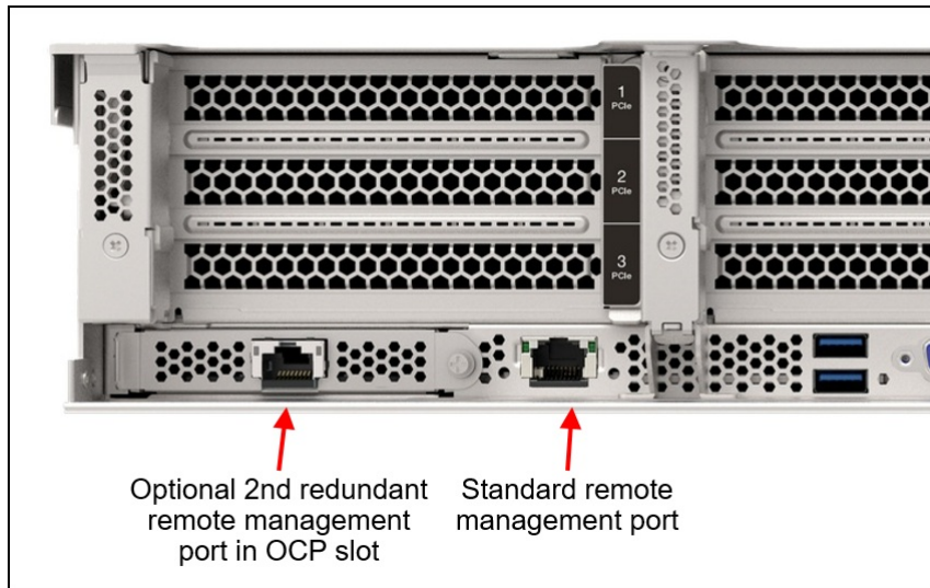
Figure 24. SR655 V3 with the Redundant System Management Port Adapter installed
