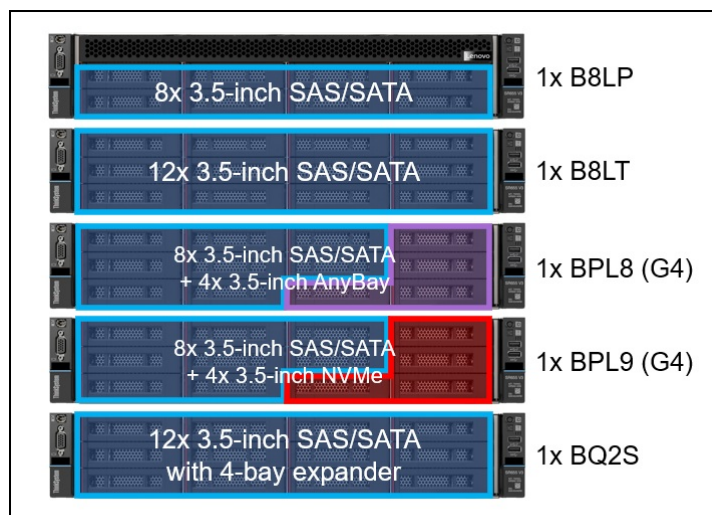
Figure 7. SR655 V3 front drive bay configurations - 3.5-inch drive bays
