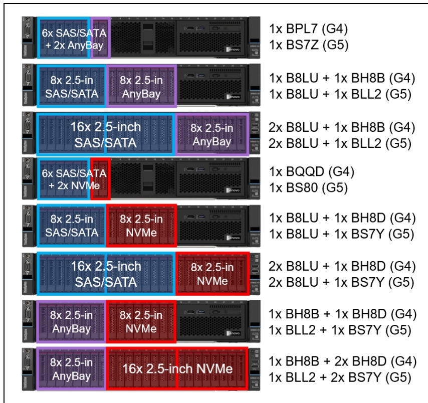
Figure 9. SR655 V3 front drive bay configurations - 2.5-inch drive bays, combinations
