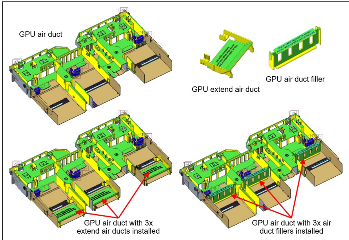
Figure 18. SR655 V3 GPU air duct
