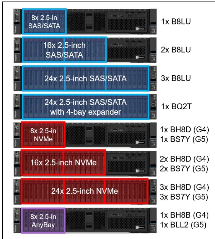
Figure 8. SR655 V3 front drive bay configurations - 2.5-inch drive bays, all the same drive type
