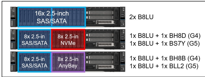
Figure 10. SR655 V3 front drive bay configurations - 2.5-inch drive bays with front PCIe slots
