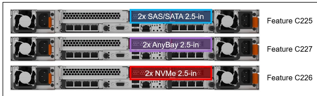
Figure 14. Rear drive bay configurations
