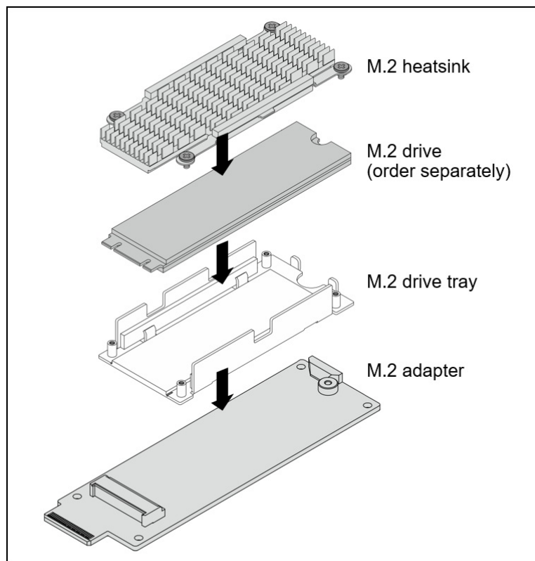
Figure 18. Components of the ThinkSystem V4 1U/2U Hot Swap M.2 SATA/NVMe Drive Assembly Kit
