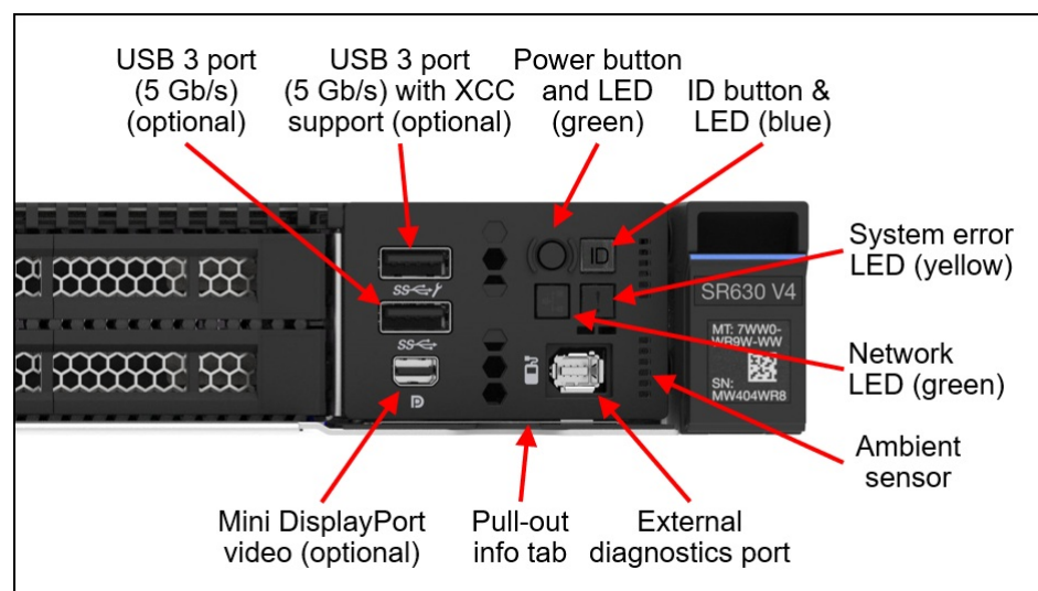
Figure 25. SR630 V4 Front operator panel
