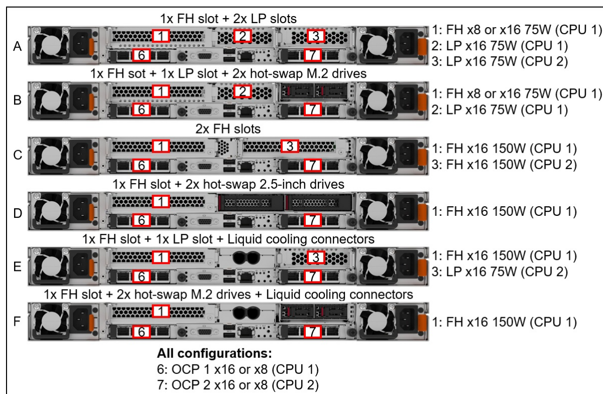
Figure 19. SR630 V4 rear slot configurations
