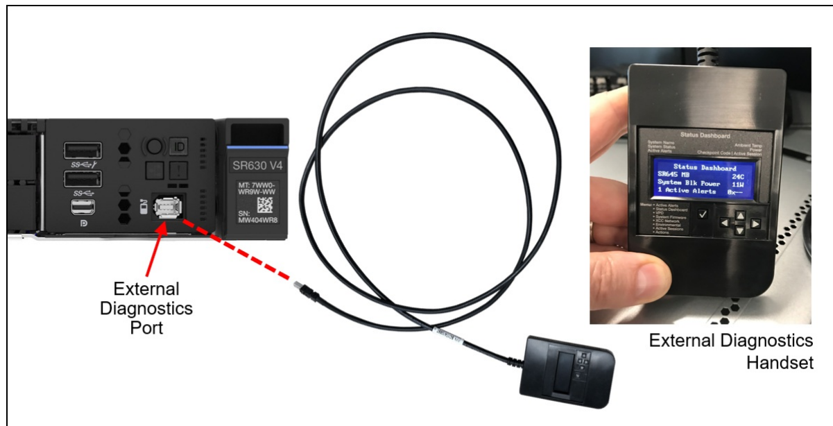
Figure 26. SR630 V4 External Diagnostics Handset
