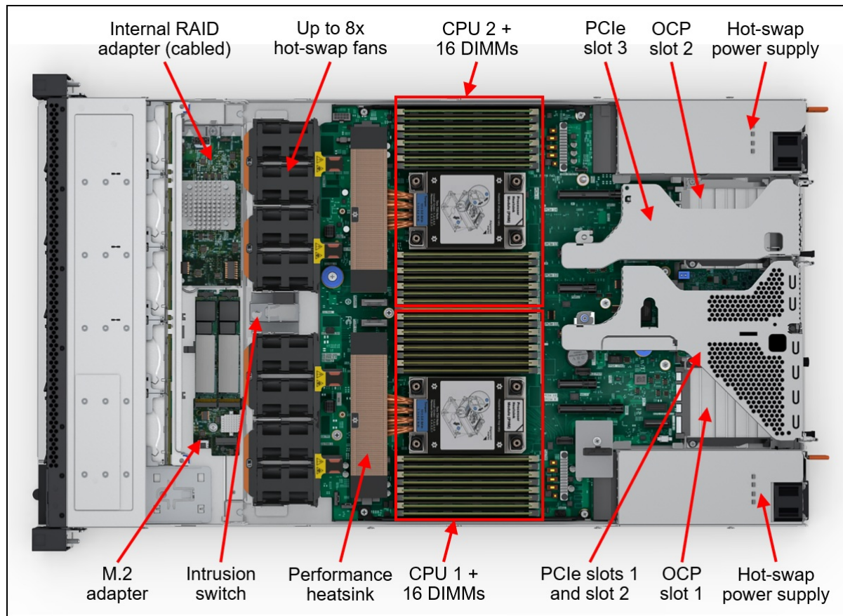
Figure 6. Internal view of the SR630 V4
