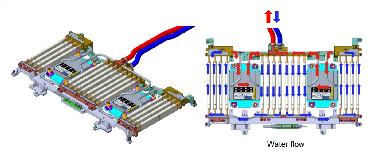
Figure 11. Lenovo Compute Complex Neptune Core Module
