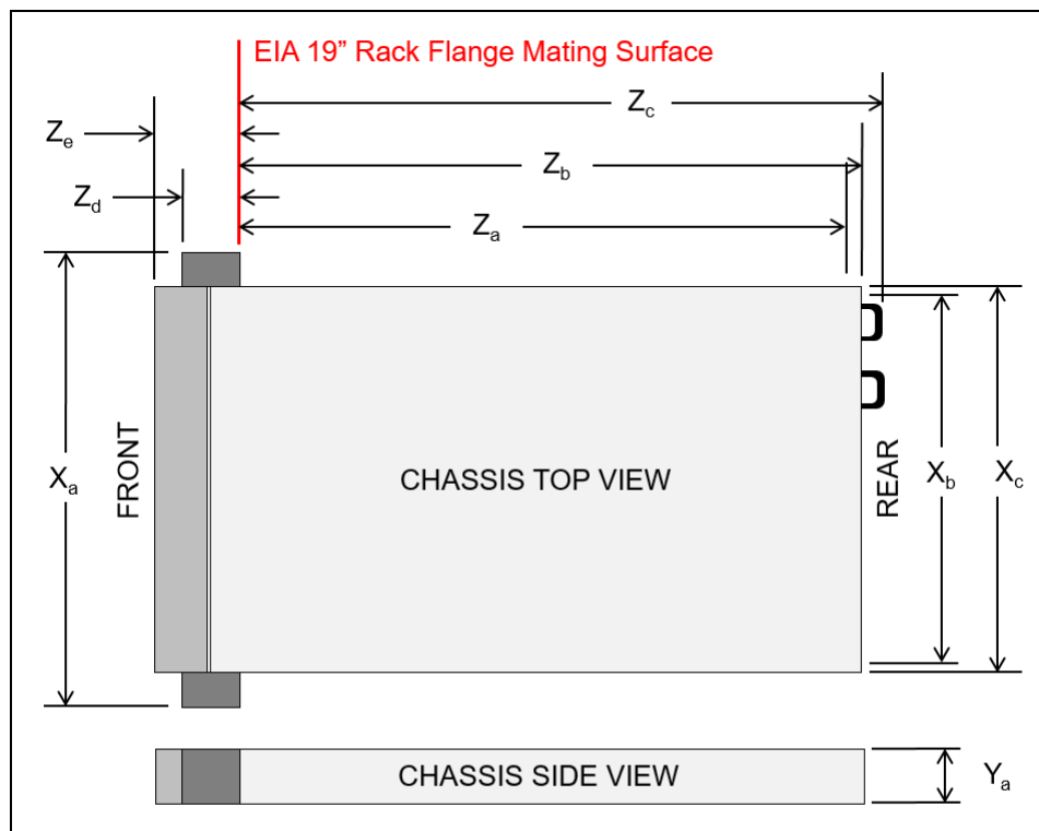
Figure 28. Server dimensions
